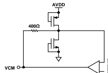
Figure 25. Equivalent VCM Circuit
