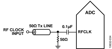
Figure 37. Typical RF Clock Input Circuit
