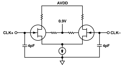
Figure 31. Equivalent Nyquist Clock Input Circuit
